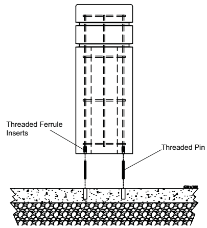
Pin and Epoxy Mount
